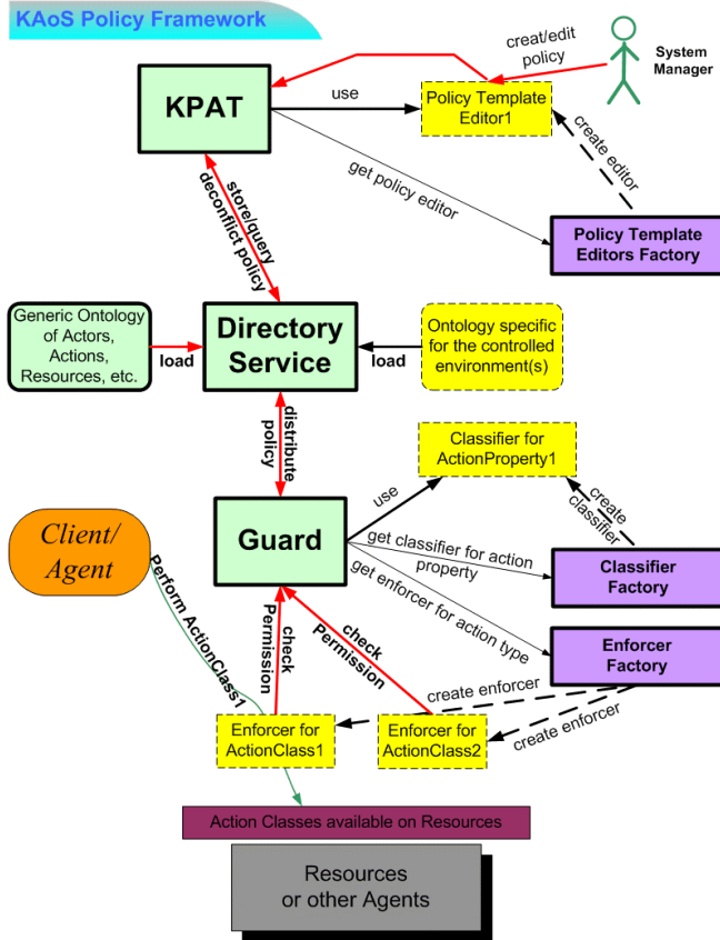
Figure 4. KAoS policy and domain services architecture.
