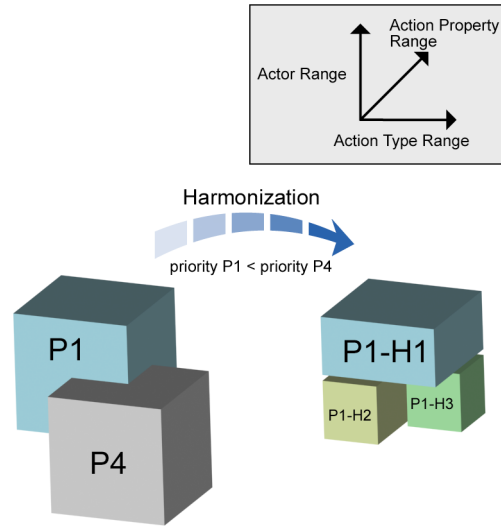
Figure 3. Graphical representation of policy harmonization.
