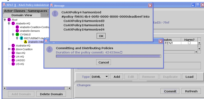
Figure 6. KPAT notifies the user of the results of policy harmonization and any issues that have arisen.
